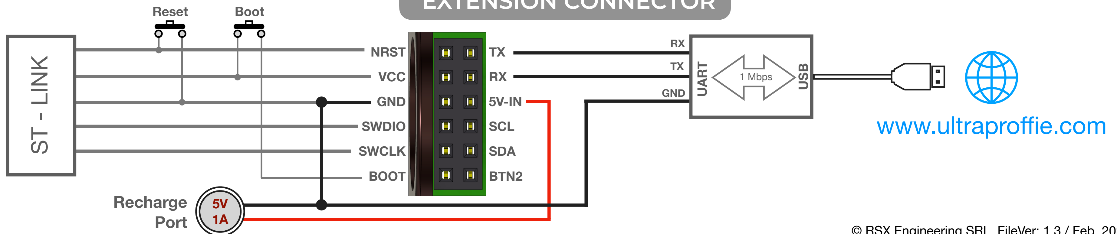
EXTENSION CONNECTOR
